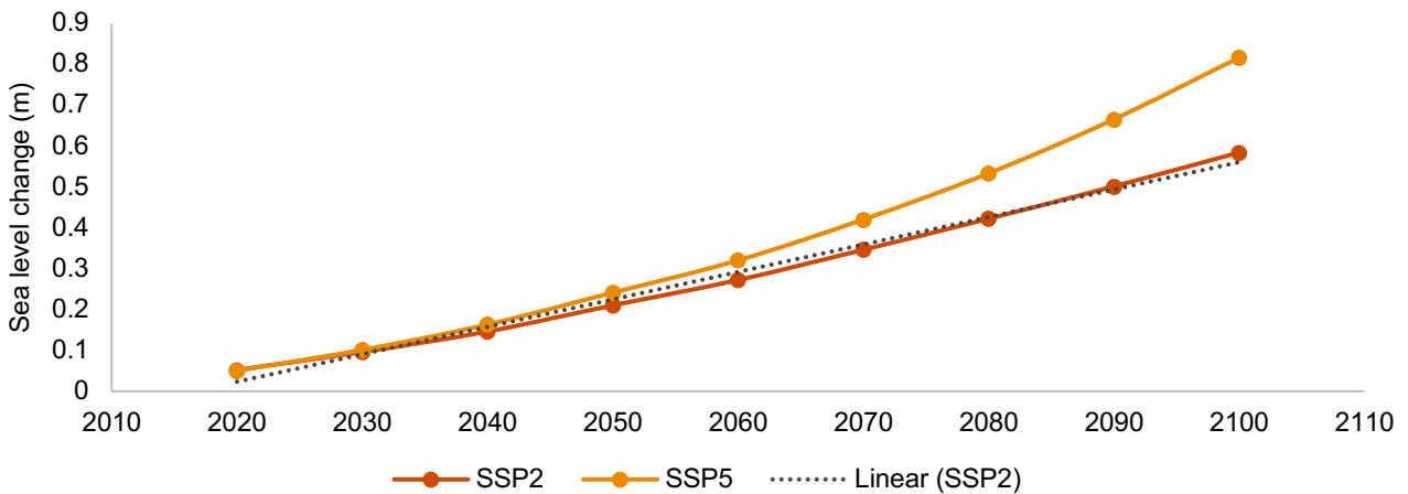
Figure 9: Projected sea level rise under different SSP scenarios
