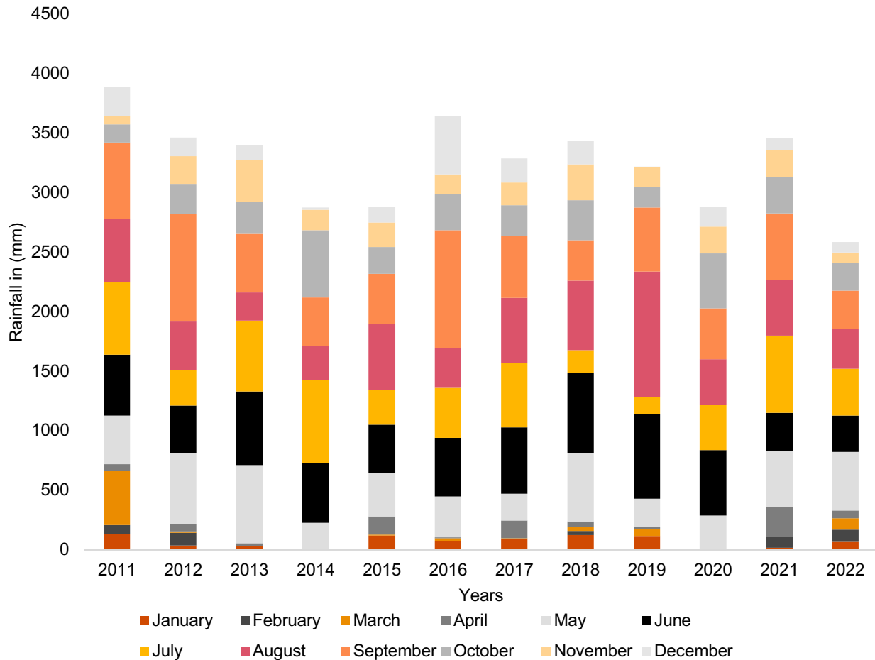
Figure 5: Rainfall recorded at Port Blair from 2011 to 2022
