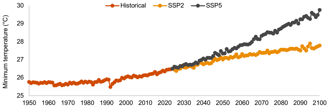
Figure 8: Minimum temperature (°C)
