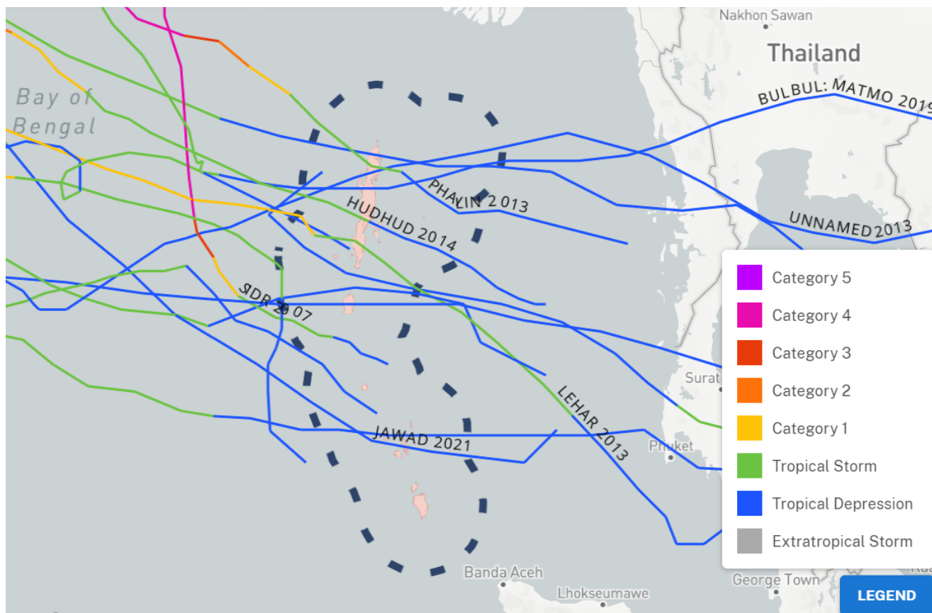
Figure 10: Cyclone tracks in the last 20 years
