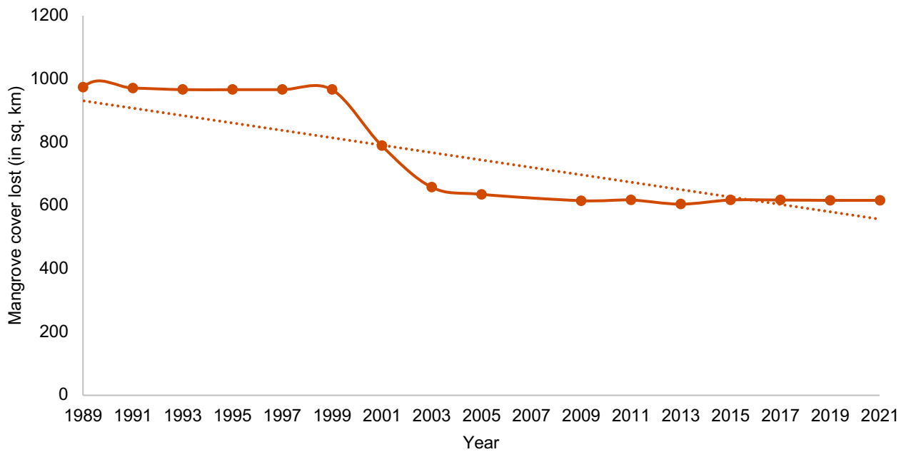
Figure 3: Mangrove loss
