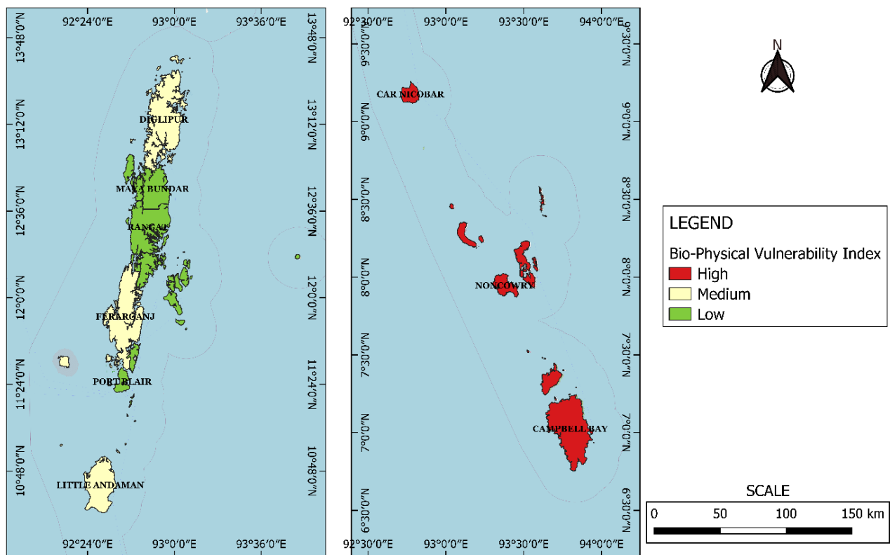
Figure 12: Map illustrating the BPVI of the ANI
